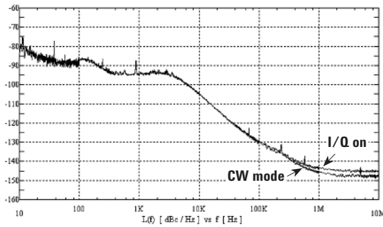
fc = 1900 MHz
